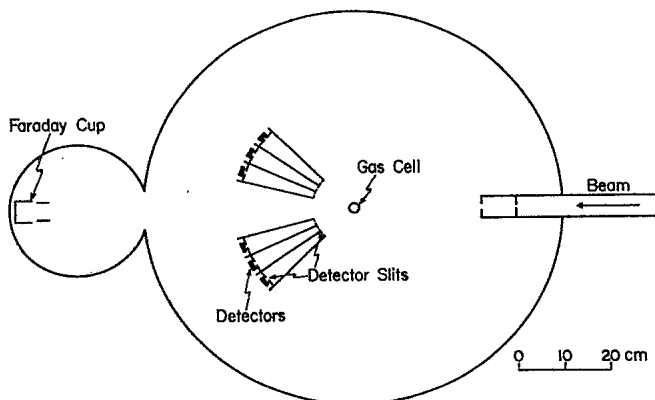
FIG. 4. Experimental setup for the {}^2\text{H}({}^6\bar{\text{Li}},\alpha){}^4\text{He} measurements.
