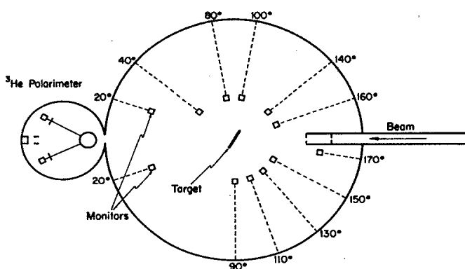
FIG. 1. Experimental setup for the ^6\text{Li}(\vec{d}, \alpha)^4\text{He} measurements.
