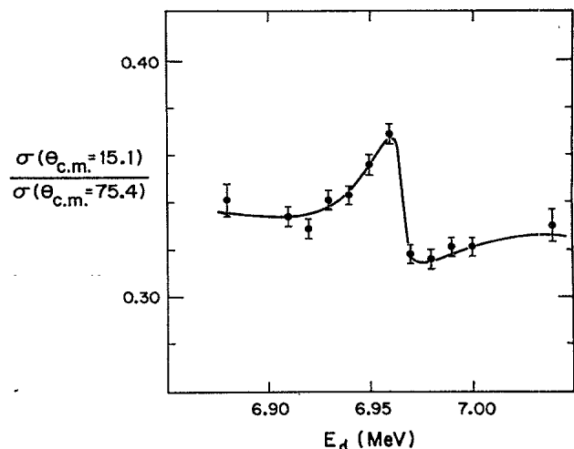
FIG. 2. Typical excitation function of \sigma(\theta_{\text{c.m.}}=15.1^\circ)/\sigma(\theta_{\text{c.m.}}=75.4^\circ) for ^6\text{Li}(d, \alpha)^4\text{He} . The curve is a guide to the eye.
